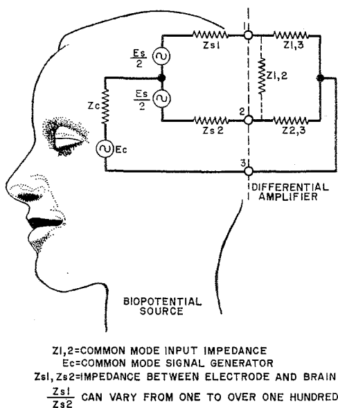
Fig. 1. Schematic of brain shows how unbalancing of source impedances ( Z_{s1} and Z_{s2} ) can affect the common mode rejection of differential circuit. Common mode generator includes all unwanted signals such as electrode potentials, power line interference, noise from extraneous body signals, etc. Unfortunately, these signals are not always common mode and show up at differential amplifier output, distorting the real brain-wave signal. Ignoring the loading effect of Z_{1,2} , and if Z_{1,3} equals Z_{2,3} , and both Z_{s1} and Z_{s2} are much less than Z_{1,3} and Z_{2,3} , the CMR limit (greatest reduction to a common mode signal) is 20 times the log to base 10 of Z_{1,3} divided by the difference between Z_{s1} and Z_{s2} . Thus, if Z_{1,3} is 100,000 ohms and electrode impedance ratio is 100, the CMR limit is 60 dB. Source and input impedance of circuit determine actual rejection. A circuit with these values produces 1 mV of common mode output noise for every 1 volt on the input.
